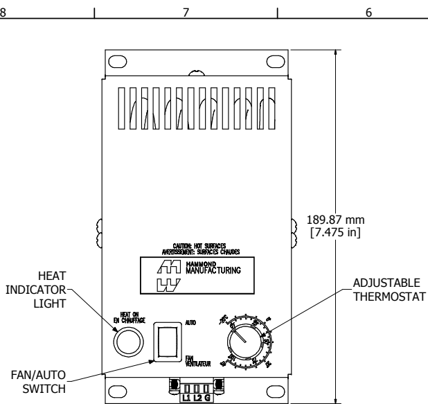
ASSEMBLY - VIEW FROM FRONT
